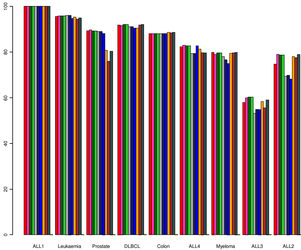
Split Sample. Training and Test. KNN classifier
