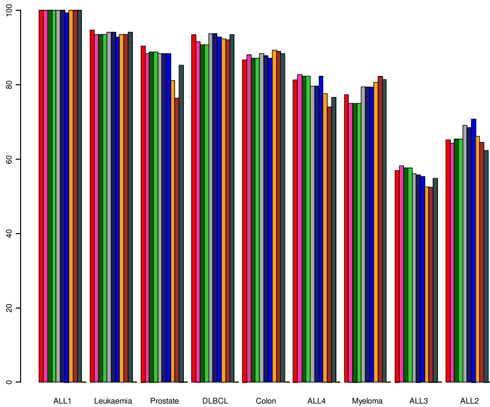
Split Sample. Training and Test. Naive Bayes classifier
