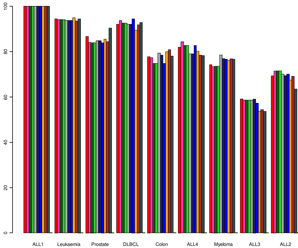
Split Sample. Training and Test. SVM classifier
