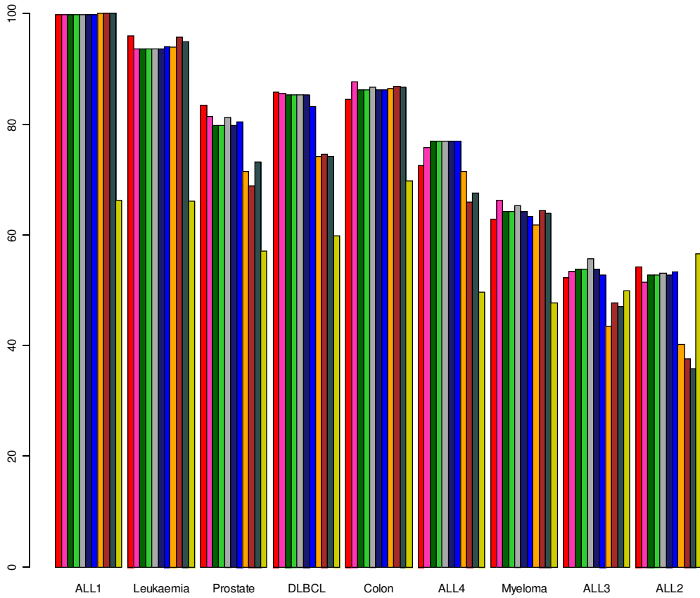
Reduced Training Set (n=10 per class). SVM classifier
