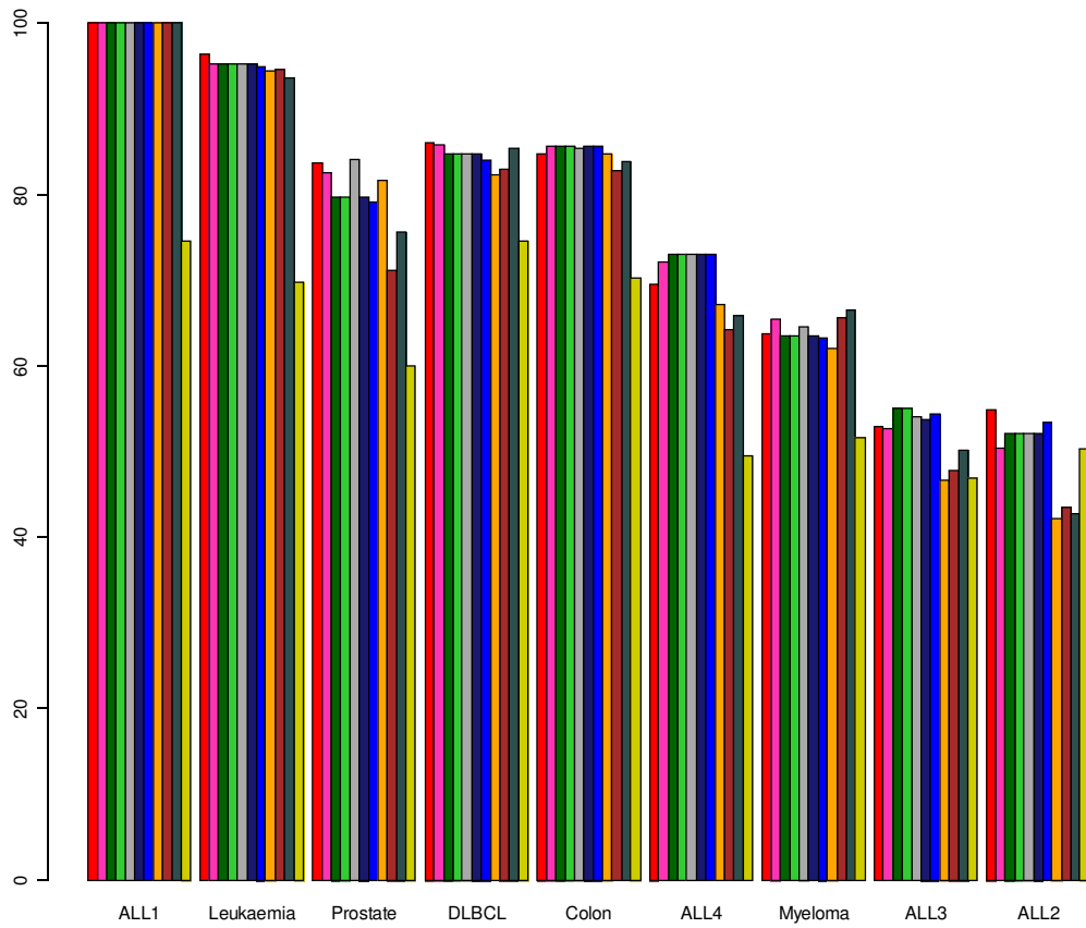
Reduced Training Set (n=10 per class). BGA classifier
