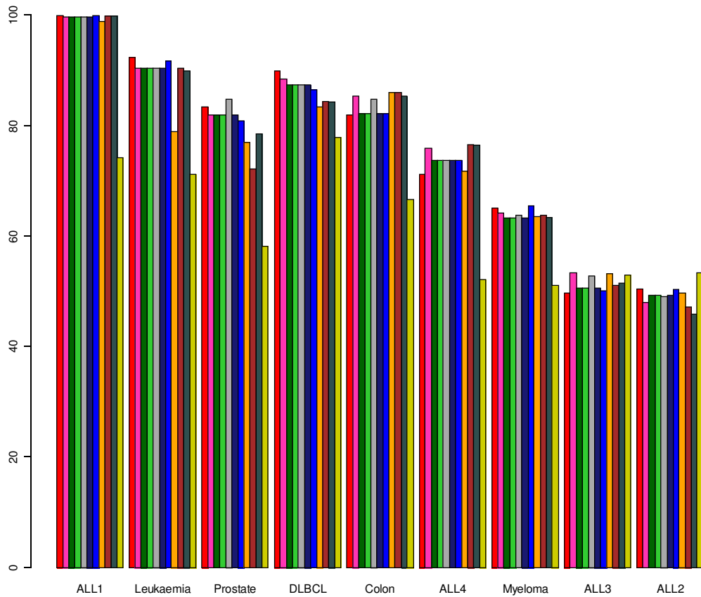
Reduced Training Set (n=10 per class). Naive Bayes classifier
