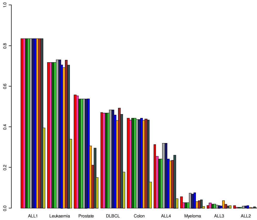
Split Sample. Training and Test. SVM classifier
