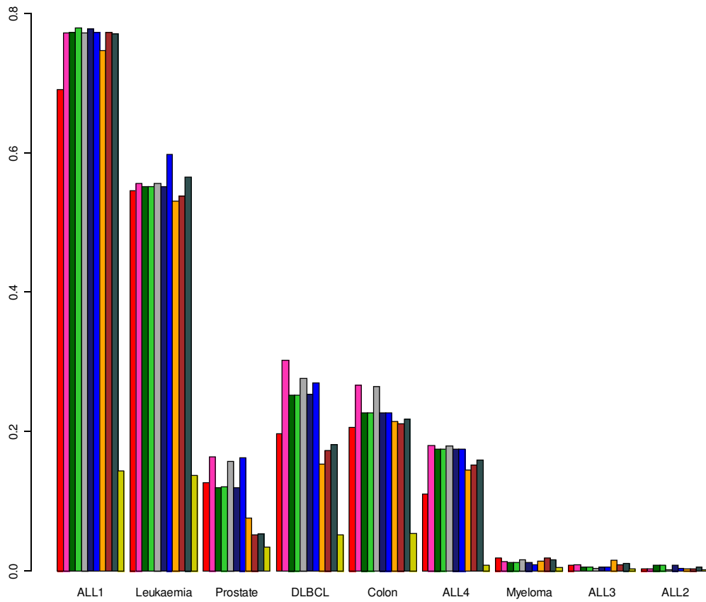
Reduced Training Set (n=5 per class). SVM classifier
