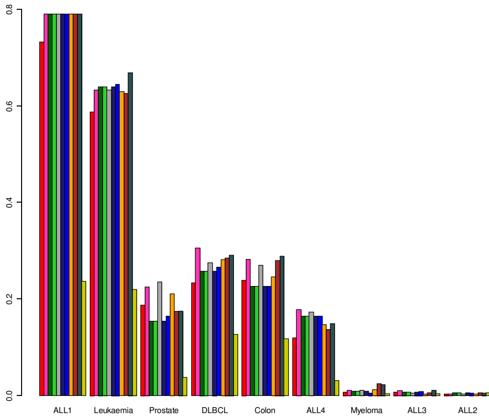
Reduced Training Set (n=5 per class). BGA classifier
