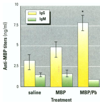
Figure 1. Antimyelin basic protein (MBP) titers (mean \pm SE) in sera of mice ( n = 6 /group) immunized with MBP and lead-altered MBP. Mice treated with lead-altered MBP show sera anti-MBP IgG titers that are significantly different from control ( *p = 0.01 ) and native MBP-immunized mice ( *p = 0.05 ). For this and all pertinent figures, IgM concentrations are reported as IgG equivalents.
