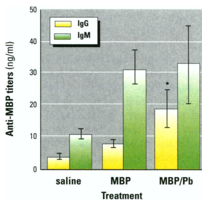
Figure 2. Antimyelin basic protein (MBP) titers (mean \pm SE) ( n = 6 /group) in lipopolysaccharide (LPS)-stimulated splenic supernatants of mice immunized with MBP and lead-altered MBP. Mice treated with lead-altered MBP show supernatant anti-MBP IgG titers that are significantly different from control mice ( *p = 0.05 ).
