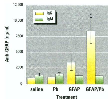
Figure 5. Antigliofibrillary acidic protein (GFAP) titers (mean \pm SE) in sera of mice ( n = 8 /group) immunized with GFAP and lead-altered GFAP. Mice treated with lead-altered GFAP show sera anti-GFAP IgG titers that are significantly different from control ( *p = 0.01 ) and lead alone ( *p = 0.01 ), and native GFAP-immunized mice ( *p = 0.05 ).
