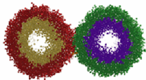
Stalk (narrow pore)
