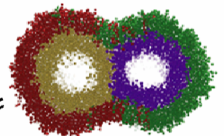
Hemifused (outer leaflet mixing)
