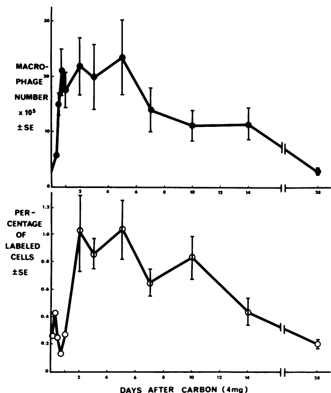
FIGURE 5. Plots of (top) the number of alveolar macrophages recovered from mouse lungs at intervals after carbon instillation and (bottom) percentages of ^3\text{H} -thymidine-labeled cells in autoradiographs. DNA synthesis in the lung is not elevated at 1 day but, from 2 days on, it correlates well with the increased number of macrophages.
