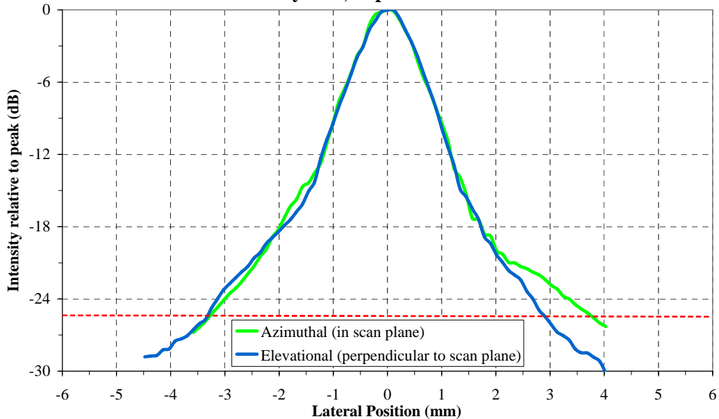
Cross Axis Intensity Plot; depth 2.5cm from transducer face
