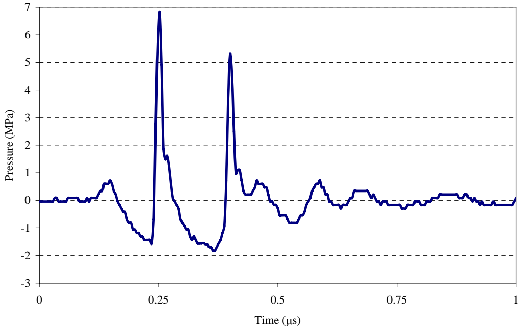
Pressure-Time Waveform at 2.5cm
