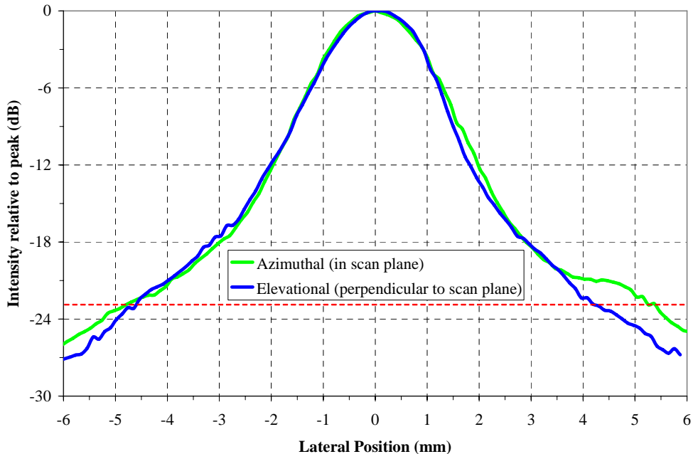
Cross Axis Intensity Plot; depth 4.5cm from transducer face
