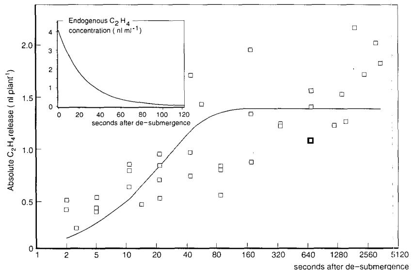
Figure 4. Ethylene release of R. palustris plotted against various desubmergence periods (seconds on a logarithmic scale) measured with laser-driven photoacoustic spectroscopy. A nonlinear fitting procedure was used and revealed the following equation: ethylene release = 1.42 (1 - e^{-0.0396t}) . Divided by the mean absolute internal gas volume of the R. palustris plants (0.349 mL), this gives a mean endogenous ethylene concentration just before desubmergence of 4.07 \text{ nL mL}^{-1} . The decline of the internal ethylene concentration in time (inset) can be expressed by the following equation: E_t = 4.07 e^{-0.0396t} .
