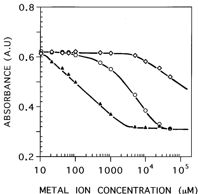
FIG. 4. A_{448} of NIT (4 µg/ml; 21 µM) at 448 nm in 0.2 M Tris-maleate buffer (pH 8.4) in the presence of different concentrations of divalent cations. Each value represents the mean of three separate experiments. Symbols: \diamond , CaCl 2 ; \circ , MgCl 2 ; \blacktriangle , MnCl 2 .
