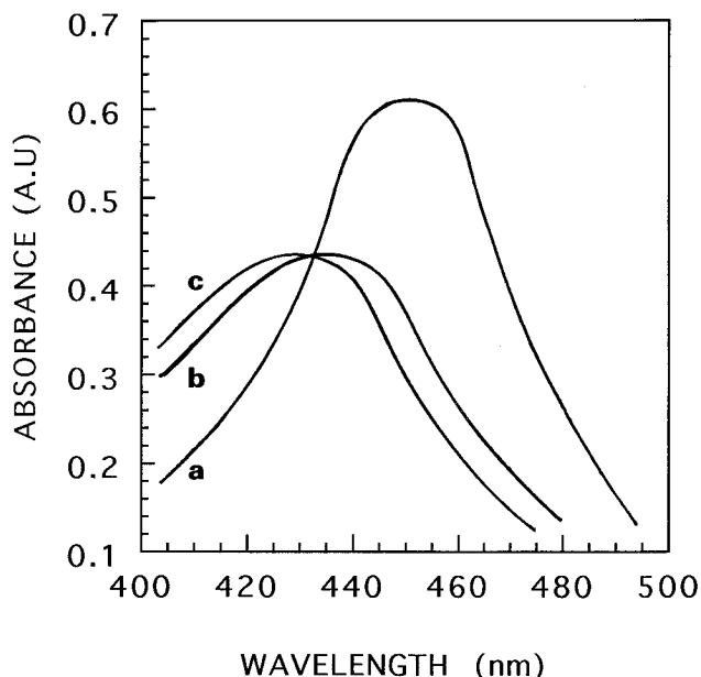
FIG. 3. Absorption spectra of NIT (4 µg/ml; 21 µM) in Tris-maleate buffer (pH 8.4). (a) NIT alone; (b) NIT in the presence of 10 mM MgCl 2 ; (c) NIT in the presence of 10 mM MnCl 2 .
