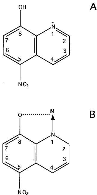
FIG. 1. Chemical structure of NIT in its unchelated form (A) and chelated form (B) with metal ion (M).
