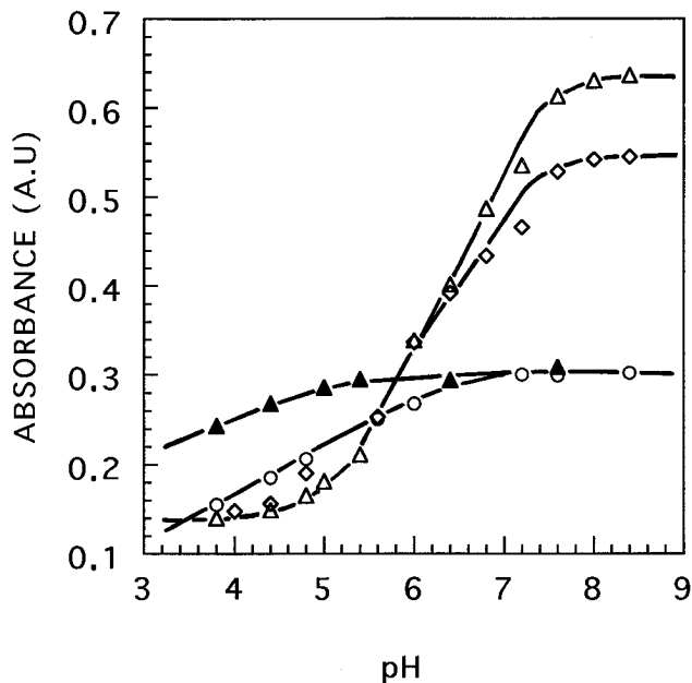
FIG. 2. A 448 of NIT (4 μg/ml; 21 μM) as a function of pH. Acetate buffer (0.1 M) was used for pHs between 3.8 and 5.6, and Tris-maleate buffer 0.2 M was used for pHs ranging from 5.2 to 8.6. Each datum point represents the mean of three experiments. Symbols: △, NIT alone or in the presence of monovalent cation (Na + , K + ); ◇, NIT in the presence of 50 mM CaCl 2 ; ○, NIT in the presence of 50 mM MgCl 2 ; ▲, NIT in the presence of 50 mM MnCl 2 .
