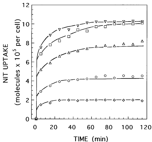
FIG. 6. Effects of external NIT concentration on NIT uptake by E. coli AL46. The uptake experiment was performed at 37°C in 50 mM sodium phosphate buffer (pH 7.2) with shaking. Saturation of NIT uptake was observed from 12 µg/ml. Each value of NIT uptake is the mean of six separate experiments. Symbols: ◇, 1 µg/ml; ○, 2 µg/ml; △, 4 µg/ml; □, 8 µg/ml; ▽, 12 µg/ml.
