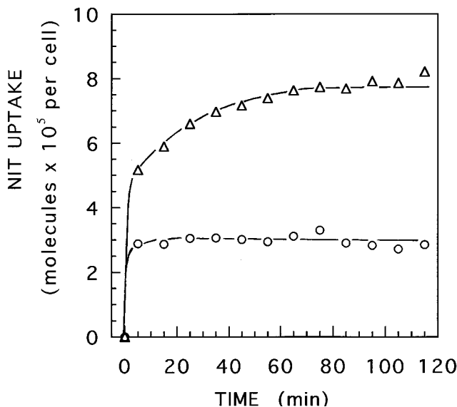
FIG. 5. Uptake of NIT (4 μg/ml; 21 μM) by E. coli AL46 as a function of incubation time. The uptake experiment was performed in 50 mM sodium phosphate buffer (pH 7.2) with shaking. Each value of NIT uptake is the mean of six separate experiments. Symbols: Δ, uptake of NIT alone at 37 or 4°C; ○, reduction in NIT uptake in the presence of 50 mM MgCl 2 preliminarily added to the cell suspension.
