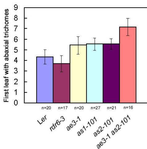
Supplemental Figure 4. Analyses of vegetative phase length of wild-type and mutants. n, plant numbers analyzed. Bars indicate standard error.
