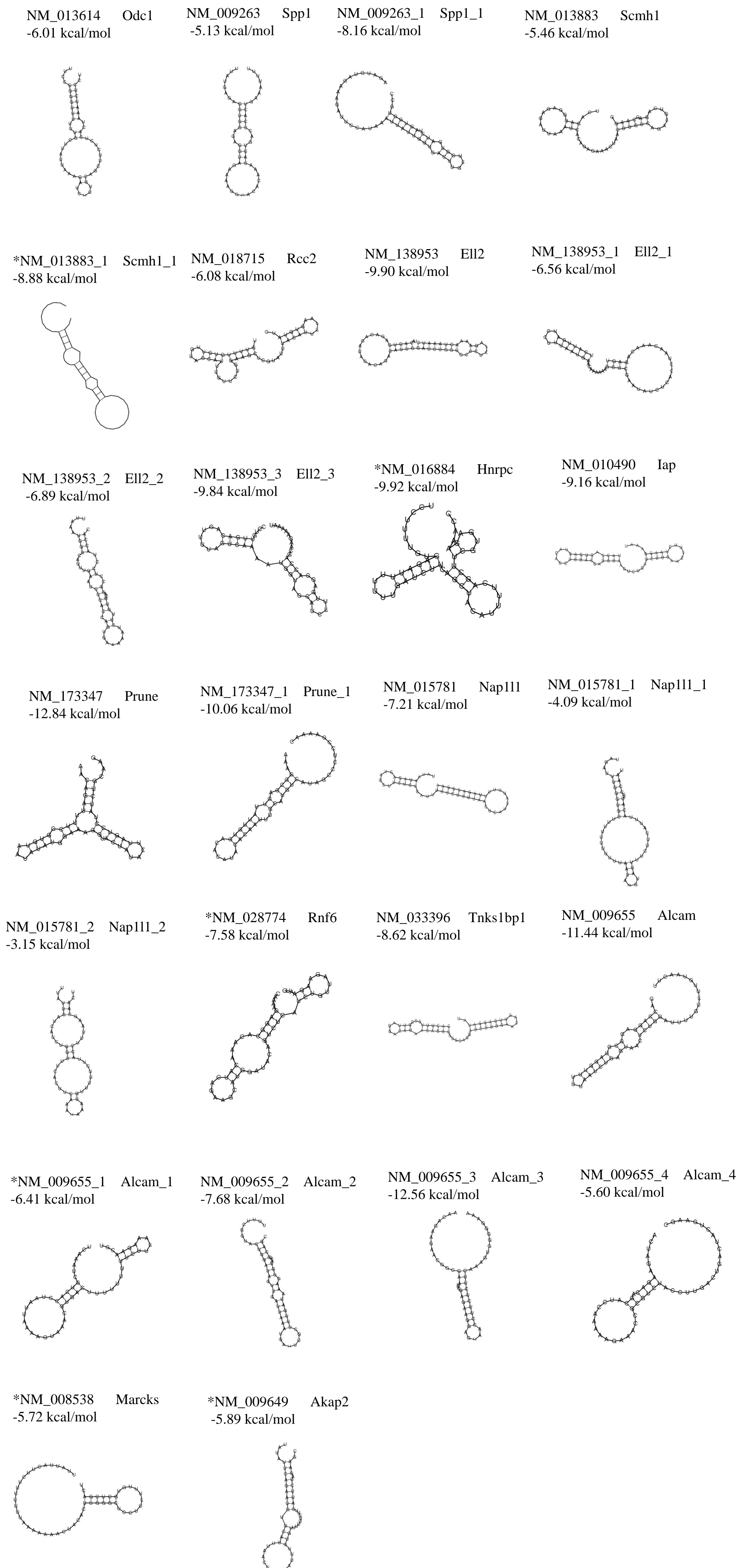
Supplement figure 1. The structures and the free energies of the 55mers predicted by RNAfold. The RefSeq IDs and the gene symbols of the transcripts are listed. The suffix indicates multiple copies of the 55mer in the same transcript. * denotes the conservation of the 55mer between mouse and human or between mouse and rat.
