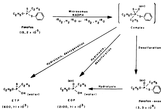
FIGURE 2. Bioactivation and inactivation mechanism of fonofos. Values in brackets denote rat oral \text{LD}_{50} (mg/kg), ( I_{50} , M ) bovine erythrocyte AChE. Data from Menn et al. (29).
