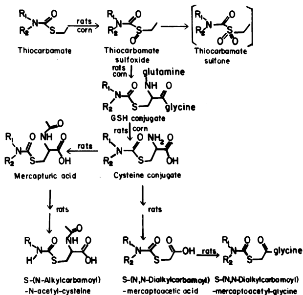
FIGURE 4. Metabolism of thiocarbamate herbicides in the rat and corn; R_1 , R_2 = propyl or isobutyl. Adapted from Hubbell and Casida (38).
