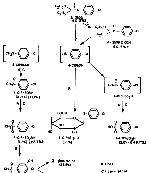
FIGURE 7. Comparative metabolism of N-2596 in the rat and corn plant. Percent values in brackets are for distribution of radiocarbon in urine; in double brackets, percent of total radiocarbon recovered in plants. Adapted from Miaullis et al. (47).
