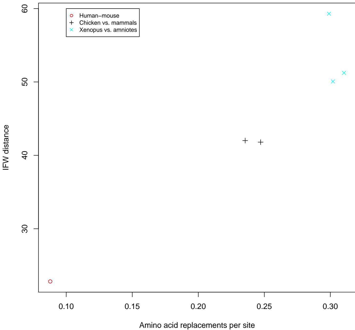
Protein diverg v. IFW distance (8bp) for promoters, mrna and EST aligning nucleotides removed
