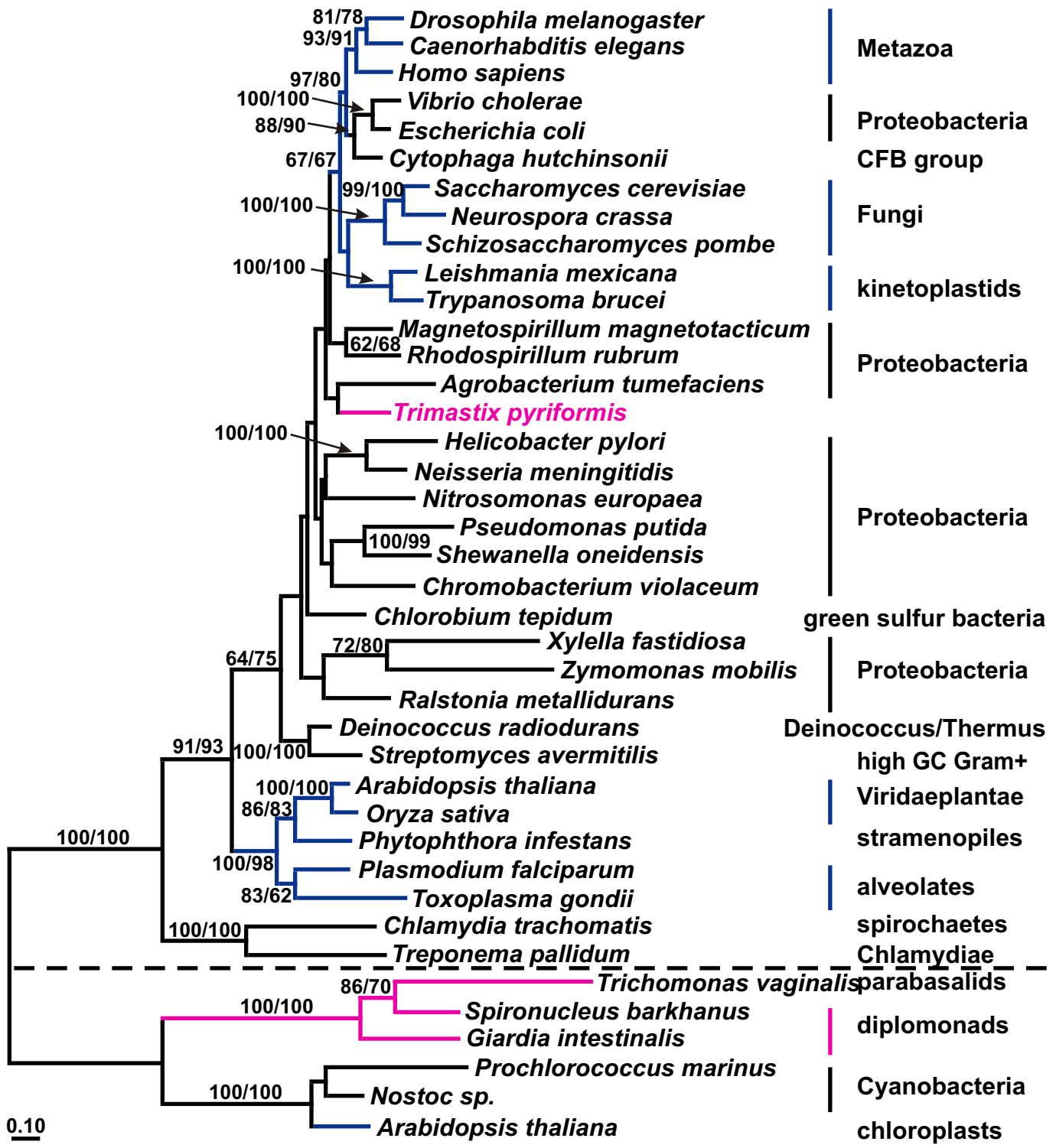
Additional File 2 - glucose-6-phosphate isomerase
