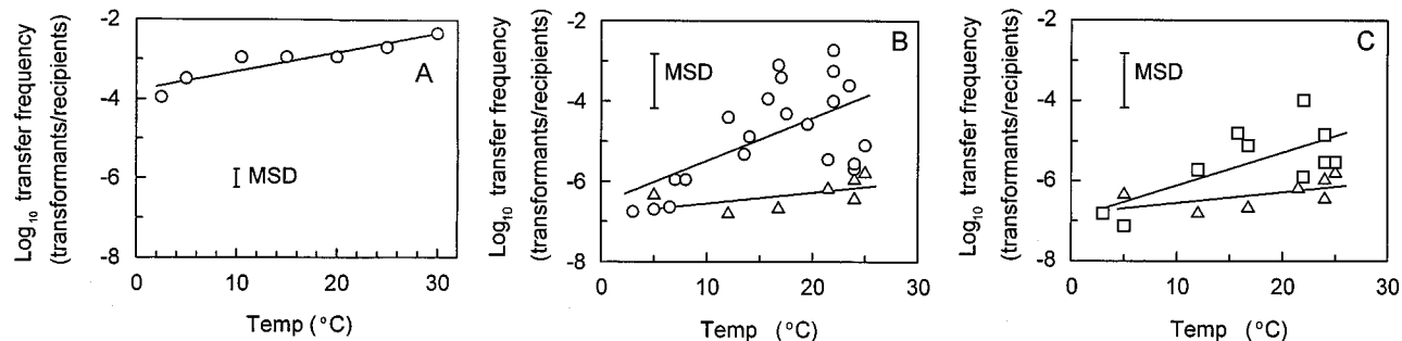
FIG. 1. Effect of temperature on transfer frequencies for HGW1521(pQM17). (A) Frequency of transfer by lysates of BD413 on PCA in the laboratory. (B) Frequency of transfer by lysates of BD413 (○) and background frequency (△) in situ. The background frequency was obtained when HGW1521(pQM17) was incubated in the river without a source of DNA. The river temperature was taken to be the median of the minimum and maximum temperatures recorded. In situ experiments at 20°C or lower were performed in the river Taff, and experiments above 20°C were performed in the Hillsborough River or the Weeki Wachee River. Each point represents the mean of three replicate experiments using different cultures incubated in the river on the same occasion. The minimum significant difference (MSD) which could be distinguished between mean transfer frequencies was 0.256 log units in the laboratory and 1.36 log units in situ.
