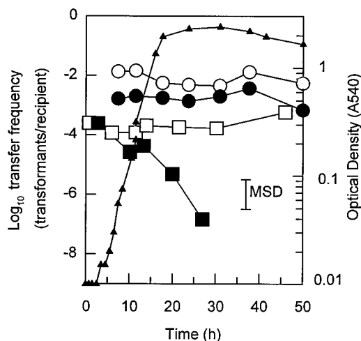
FIG. 2. Effect of culture age on transformation. Cultures of HGW1521 (pQM17) grown between 15 min and 50 h were transformed to prototrophy by lysates of BD413 in the laboratory at 20°C on PCA (●) at 20°C on B22 salts agar (○) and at 5°C on B22 salts agar (□) or in the Hillsborough River (■) at \approx 23.5^\circ\text{C} . The optical density of the recipient cultures was measured at 540 nm (▲). MSD, minimum significant difference.
