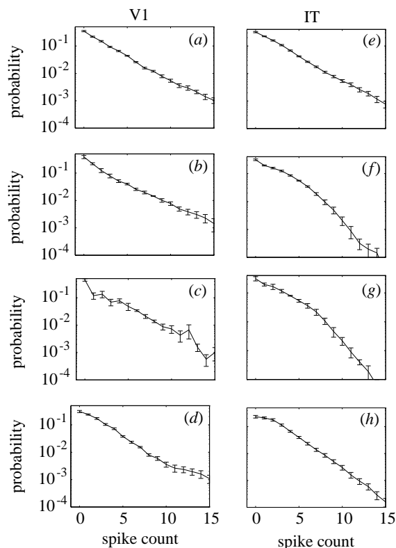
Figure 4. Spike-count distributions for six different video conditions and two noise conditions. In each case the window size was chosen so that the average number of spikes per window was one. Near exponential spike count distributions were found for all three video conditions: mixed (a), natural (b), indoor (c), laboratory (e), colony (f) and artificial (g). More surprisingly, the white noise (d), and blank screen (h) conditions also produced approximately exponential distributions. Error bars correspond to standard errors.
