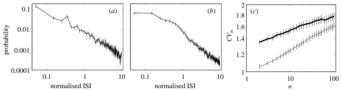
Figure 5. Normalized ISI distributions, and CV_n as a function of n . For each cell, the distribution of interspike intervals was found, the intervals were divided by the average ISI for each cell and the resulting normalized ISI distributions were averaged over all cells. Results are shown for video stimulated cat V1 cells (a) and macaque IT cells (b), with the error bars corresponding to standard errors. Both are plotted on log-log axes. (c) CV_n as a function of n . The thick line indicates the result for cat V1 and the thin line is for monkey IT.
