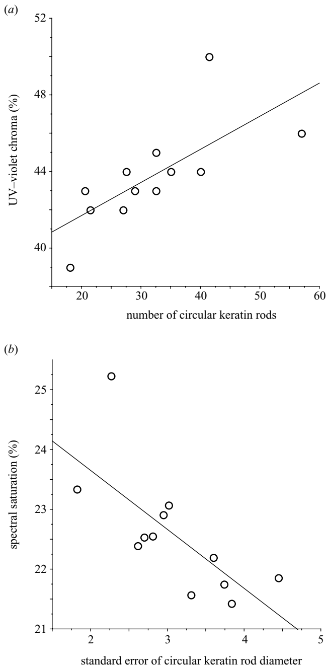
Figure 5. Scatterplots of colour variables versus nanostructural variables of feather barbs from male eastern bluebirds. Colour was measured from intact feathers, whereas nanostructure was measured from 1024 \text{ pixel} \times 1024 pixel sections of TEM micrographs of the barbs' spongy layer. (a) Scatterplot of UV-V chroma versus the number of circular keratin rods. (b) Scatterplot of spectral saturation versus the standard error of circular keratin rod diameter. Stepwise linear regressions: (a) r^2 = 0.462 , p = 0.016 . (b) r^2 = 0.498 , p = 0.010 . n = 12 in all cases.
