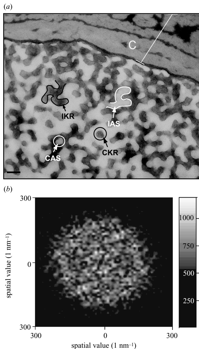
Figure 3. (a) Transmission electron micrograph ( \times 25\,000 ) of the spongy layer of a contour feather from a male eastern bluebird. Abbreviations: C, cortex; IKR, irregular keratin rod; IAS, irregular air space; CKR, circular keratin rod; CAS, circular air space. Scale bar, 100 nm. (b) Two-dimensional Fourier power spectrum of TEM of colour-producing spongy layers of eastern bluebirds. The length and direction, respectively, of a vector from the origin to each value in the power spectrum indicates its spatial frequency and direction (for more details, see Prum et al. 1999a). The colour indicates the magnitude of each value in the power spectrum (scale on right).
