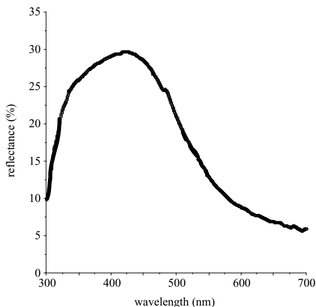
Figure 1. Typical reflectance spectra of rump feathers from a male eastern bluebird.
