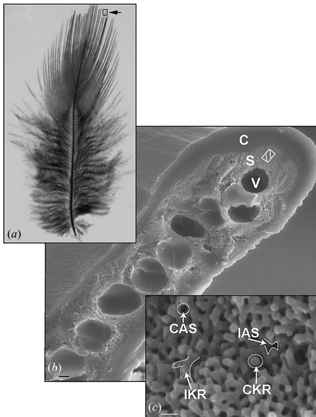
Figure 2. (a) A rump feather from a male eastern bluebird. The box around the tip of the barb indicates the region sectioned for SEM and TEM examination. (b) SEM ( \times 1000 ) of barb cross-section. The hatched box at the most distal region of the barb is enlarged in (c). Scale bar, 4 \mu\text{m} . (c) SEM ( \times 20\,000 ) of the spongy region (S) directly under the cortex (C), but above the vacuoles (V) of the feather barb. The nanostructural components outlined include an irregular keratin rod (IKR), circular keratin rod (CKR), irregular air space (IAS) and circular air space (CAS). Scale bar, 80 nm.
