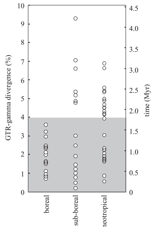
Figure 3. Genetic distances (GTR-gamma distances) and approximate dates of coalescence events between closely related species belonging to superspecies in boreal forest, sub-boreal and neotropical lowland avifaunas. The Pleistocene is indicated by the shaded area.
