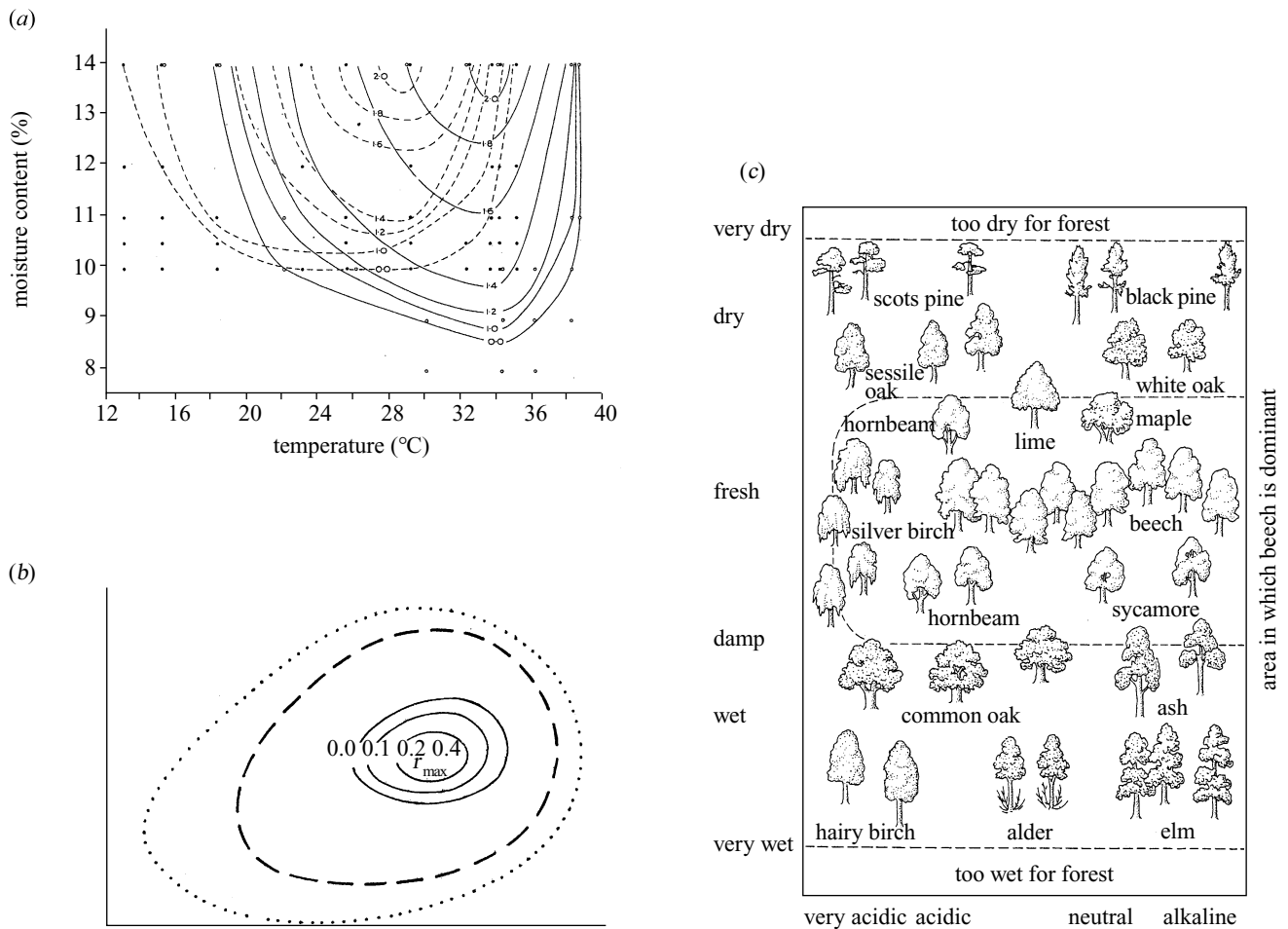
Figure 2. The ecological niche defined by population growth rate contours. (a) The study by Birch (1953) of the effects of temperature and wheat moisture content on population growth rate = \lambda of two species of grain beetle: dotted lines, Calandra oryzae ; solid lines, Rhizopertha dominica . The points on the graph show conditions at which measurements were made. (b) Maguire's (1973) definition of the ecological niche in terms of population growth rate = r contours (after Hutchinson 1978). Axes are environmental variables as described in the text. (c) Niches of the major northern European trees. (From Polunin & Walters (1985), copyright owned by Ellenberg (1988).)
