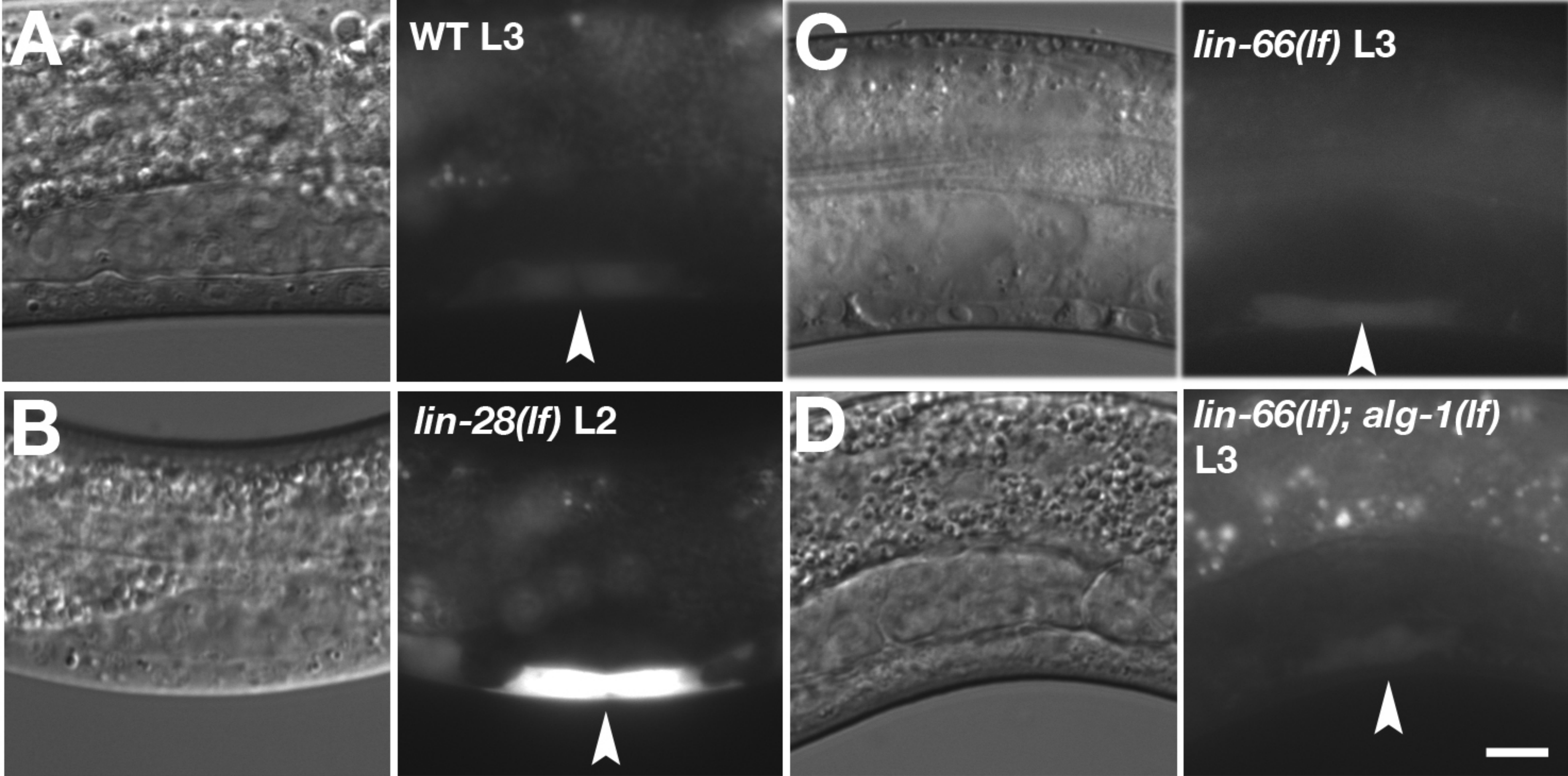
Figure S2. egl-17::GFP expression in heterochronic gene mutants DIC (left) and fluorescent (right) images of WT and mutant animals at L2 or L3 stages as indicated. Arrows indicate the egl-17::GFP expression in the P6.p cell.
