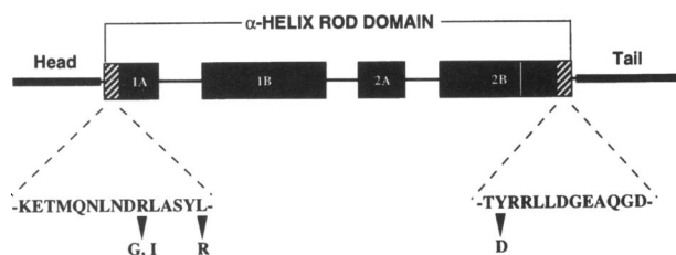
Figure 4 Depiction of the domain structure of K12 and the mutations found in MCD. The rod domain comprises \alpha -helical segments 1A, 1B, 2A, and 2B, flanked by the nonhelical head and tail domains. The vertical line in the middle of segment 2B represents the "stutter" that is an interruption in the phasing of the heptad repeat. The helix-initiation and -termination motifs are denoted by hatched boxes at the beginning and end of the rod domain, respectively. The amino acid sequences for the helix-initiation and -termination motifs are shown.
