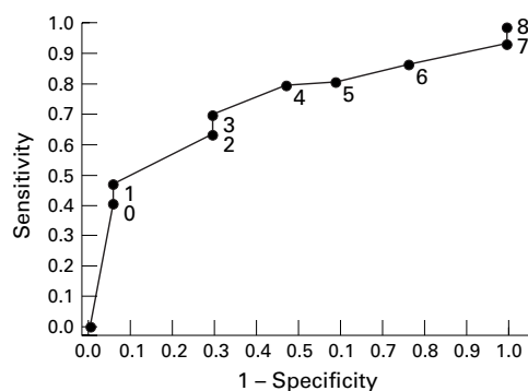
Figure 2 ROC curve for various post-treatment dyspepsia scores for predicting eradication of H pylori .
