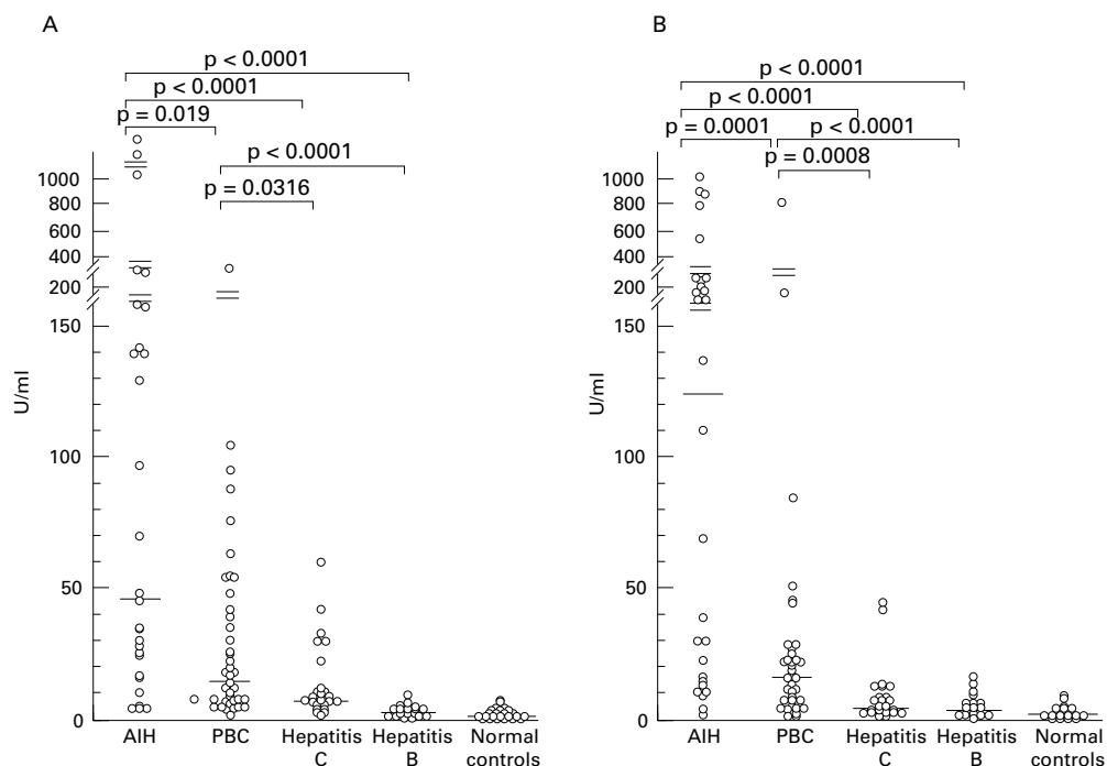
Figure 2 Titres of antibodies to HMG1 (A) and HMG2 (B) determined by ELISA. AIH, autoimmune hepatitis; PBC, primary biliary cirrhosis. The solid lines represent median values of antibody titres. p values by Mann-Whitney U test.
