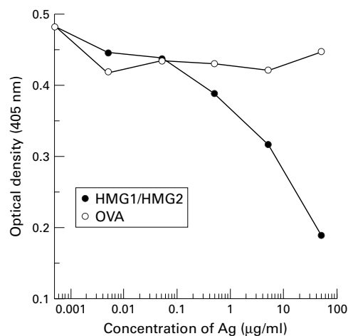
Figure 3 Competitive inhibition ELISA. Anti-HMG1/HMG2 antibody positive serum from a patient with autoimmune hepatitis was preincubated with a mixture of HMG1 and HMG2 or ovalbumin (OVA) at the concentrations indicated. In a subsequent HMG1/HMG2 ELISA, the reactivity decreased in a dose dependent manner when preincubated with HMG1/HMG2, but not with ovalbumin.
