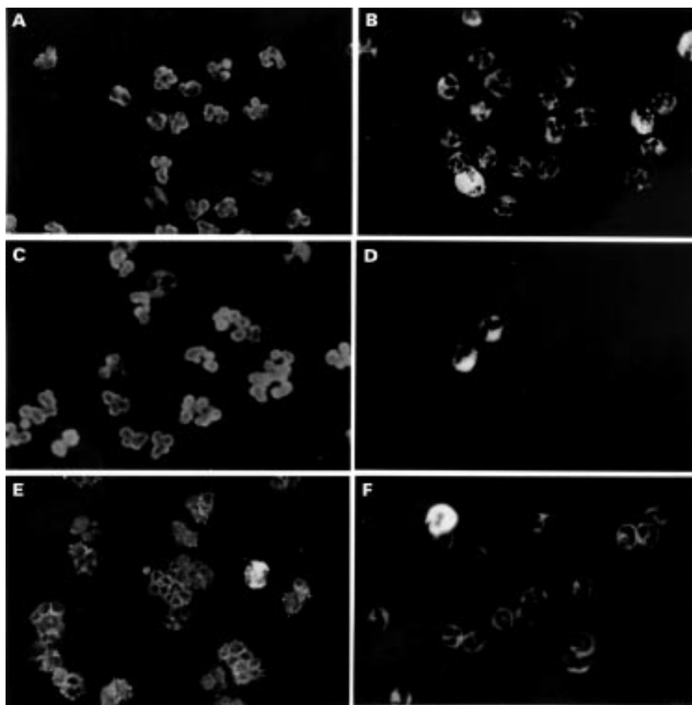
Figure 1 Perinuclear anti-neutrophil cytoplasmic antibody activities on indirect immunofluorescence. Sera from patients with autoimmune hepatitis (A, B) and primary biliary cirrhosis (C, D), and an affinity purified anti-HMG1/HMG2 antibody (E, F) showing perinuclear staining on ethanol fixed neutrophils (A, C, E) and cytoplasmic or negative staining on formalin fixed neutrophils (B, D, F).
