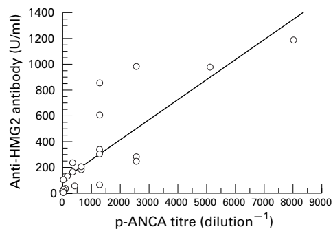
Figure 4 Correlation between the titres of anti-HMG2 antibody and perinuclear anti-neutrophil cytoplasmic antibodies in autoimmune hepatitis. A positive correlation was found between the two parameters ( r = 0.8264 , p < 0.0001 , Spearman rank correlation test).
