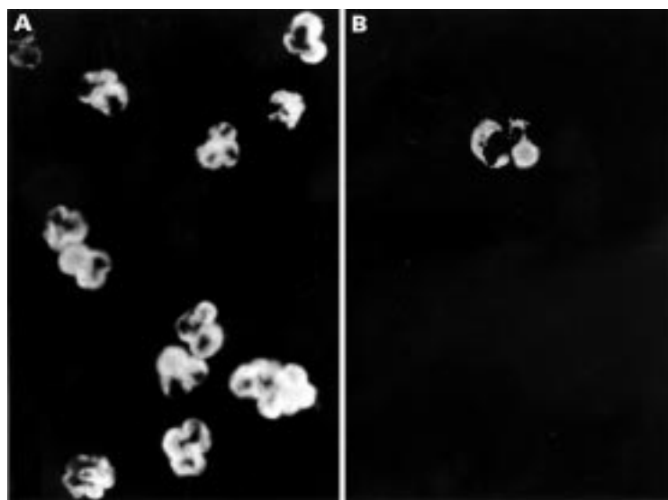
Figure 5 Disappearance of perinuclear anti-neutrophil cytoplasmic antibody (p-ANCA) staining after preincubation with specific antigens. Serum from a patient with autoimmune hepatitis with a p-ANCA titre of 1280 was diluted at 1:160 and preincubated with an equal volume of 100 µg/ml of a mixture of HMG1 and HMG2 (B) or phosphate buffered saline (A). Subsequent IIF was performed by each solution, and photographs were taken at the same exposure. No fluorescence was visible in (B), where the only bright cell is an eosinophil with spontaneous fluorescence.
