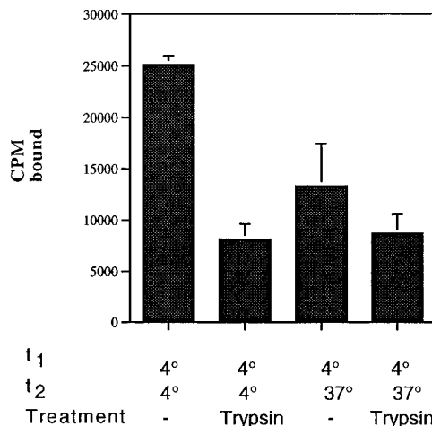
FIG. 5. Binding and internalization of ^{125}\text{I} -SLT-I by undifferentiated THP-1 cells. Radioiodinated SLT-I was incubated with 5 \times 10^6 cells per ml at 4^{\circ}\text{C} for 1 h ( t_1 ). Unbound toxin was removed by washing, and the cells were either maintained at 4^{\circ}\text{C} or shifted to 37^{\circ}\text{C} for 1 h ( t_2 ). Cells were treated with trypsin for 15 min at room temperature or not treated with trypsin (-). Binding of ^{125}\text{I} -SLT-I to cells was quantitated by scintillation counting.
