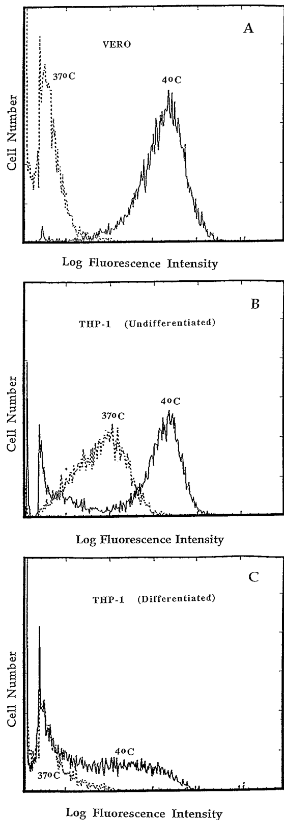
FIG. 4. Internalization of SLT-I by THP-1 and Vero cells. Cells ( 10^6 cells per ml) were incubated with purified SLT-I for 1 h at 4^{\circ}\text{C} . After three washes with ice-cold buffer, some cells were incubated at 37^{\circ}\text{C} to allow internalization and other cells were maintained at 4^{\circ}\text{C} . Cell-bound toxin was detected by flow cytometry as described in Materials and Methods. The graphs shown are representative of five independent experiments.
