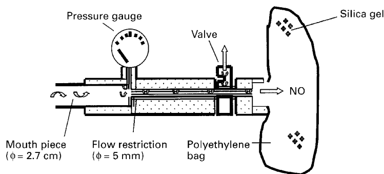
Figure 1 Schematic diagram of the portable equipment for collection of exhaled NO. The arrows indicate the direction of air flow. The three way valve is in the closed position for reservoir collection of exhaled breath.
