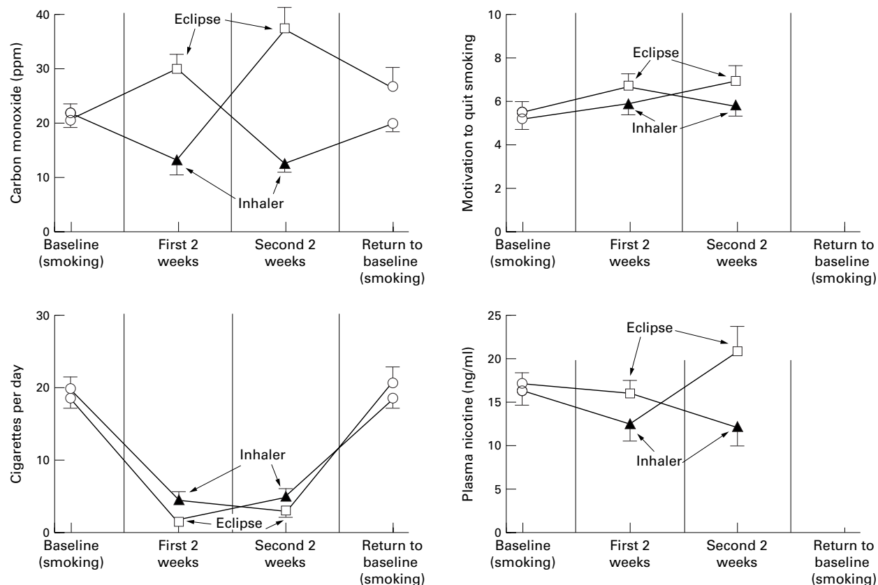
Figure 2 Baseline, treatment, and return to baseline values for number of cigarettes smoked per day, carbon monoxide concentration, plasma nicotine concentration, and motivation to quit smoking.
