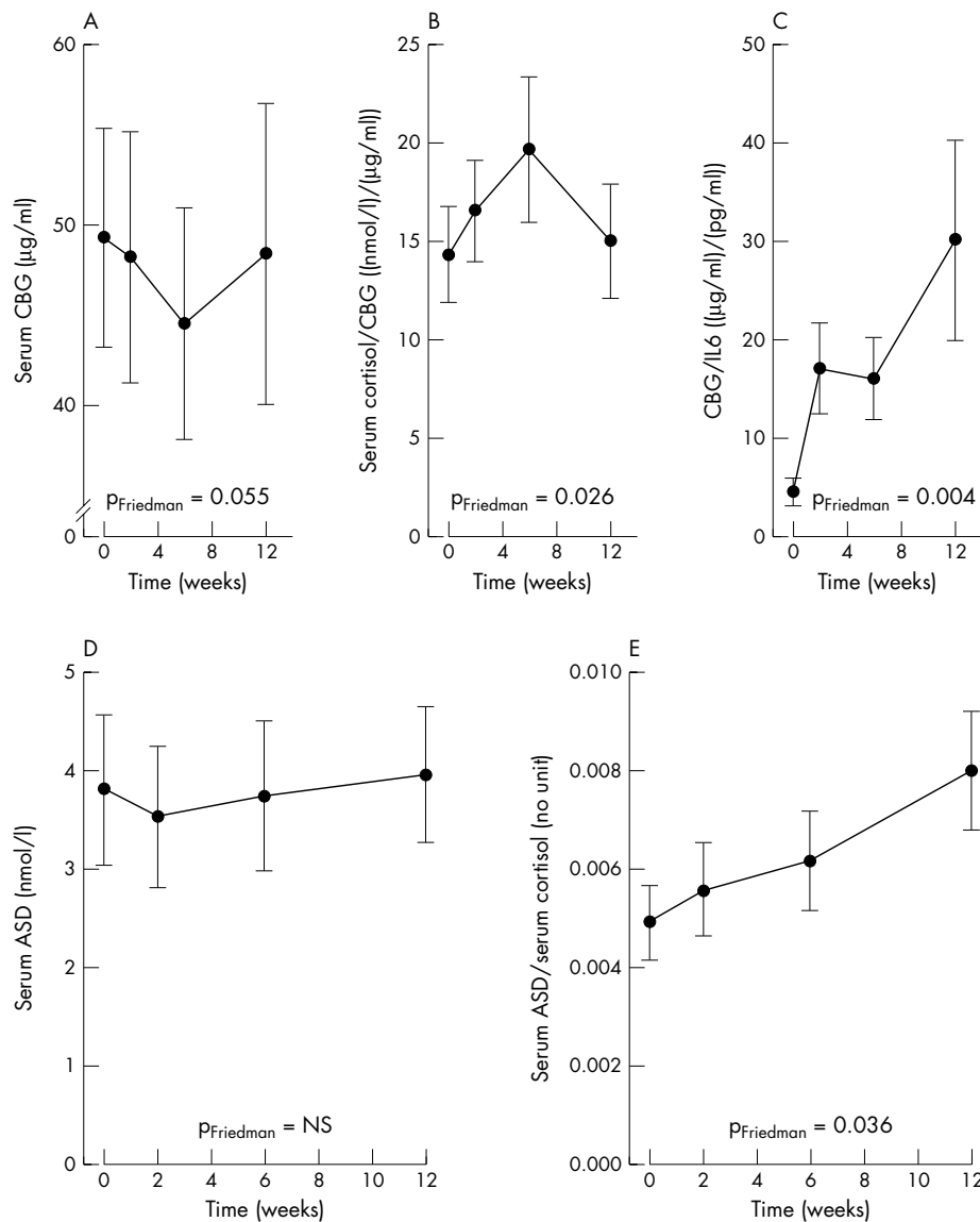
Figure 1 Course of serum cortisol binding globulin (CBG) and androstenedione (ASD) in relation to cortisol during 12 weeks of anti-TNF antibody treatment in patients with RA. Baseline values are given as time point 0. The graph depicts serum CBG (A), the ratio serum cortisol/CBG (B), the ratio serum CBG/IL6 (C), serum ASD (D), and the ratio serum ASD/cortisol (E). The data are given as means (SEM). The p value according to Friedman's test is given.
