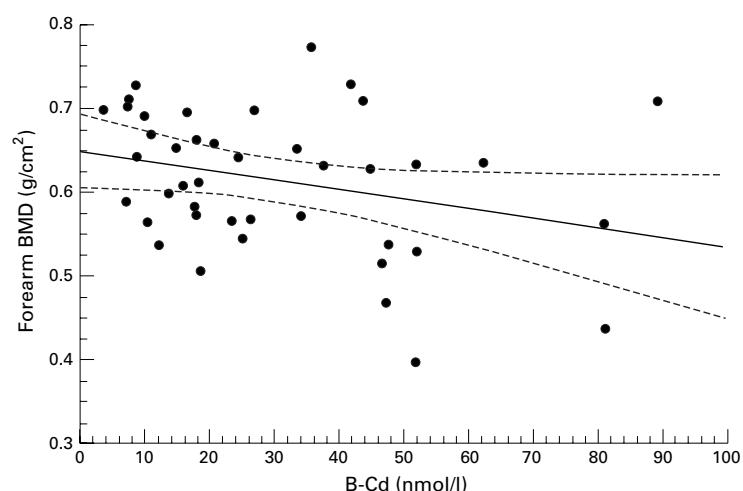
Figure 3 Forearm bone mineral density as a function of B-Cd in workers exposed to cadmium.
