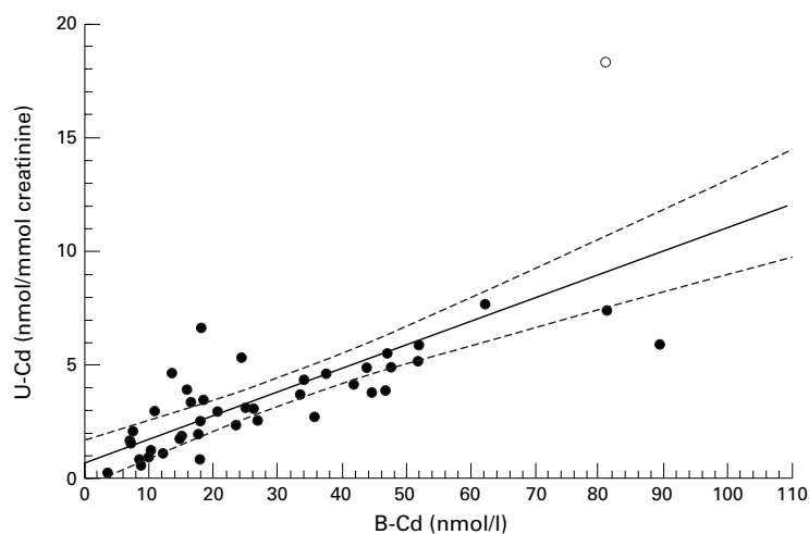
Figure 2 Urinary cadmium measured in 1993 as a function of B-Cd measured in 1996.
