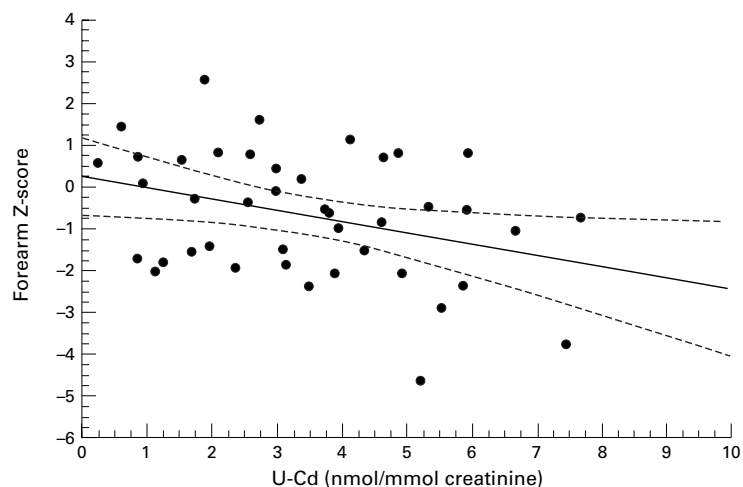
Figure 4 Forearm Z score as a function of U-Cd in workers exposed to cadmium.
