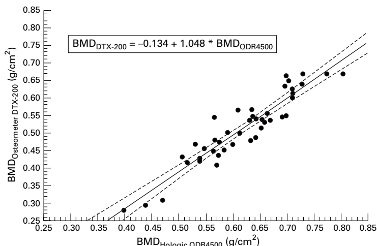
Figure 1 Forearm bone mineral density (BMD) in solderers exposed to cadmium, measured by a movable instrument (Osteometer DTX-200) as a function of forearm BMD measured by a hospital based instrument (Hologic QDR 4500).
