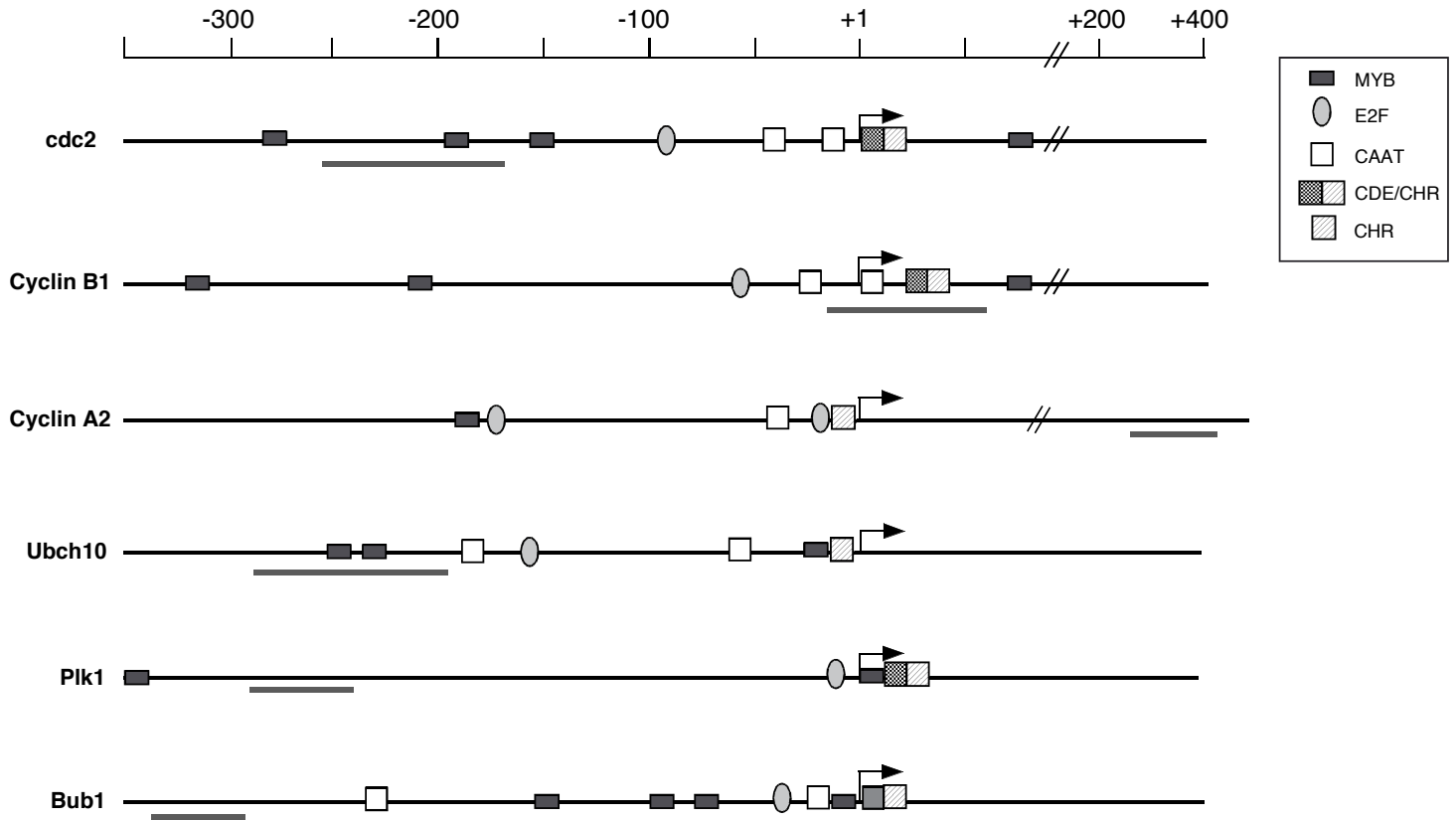
Figure S3: Schematic overview of LIN-9 regulated G2/M promoters. Potential binding sites for E2F and B-MYB are indicated. CAAT Boxes, CDE/CHR elements and isolated CHR elements are also shown. Transcription factor binding sites are based on published studies or were identified by comparison with consensus binding sequences. Grey lines indicate real-time PCR amplicons amplified in Chromatin Immunoprecipitation assays.
