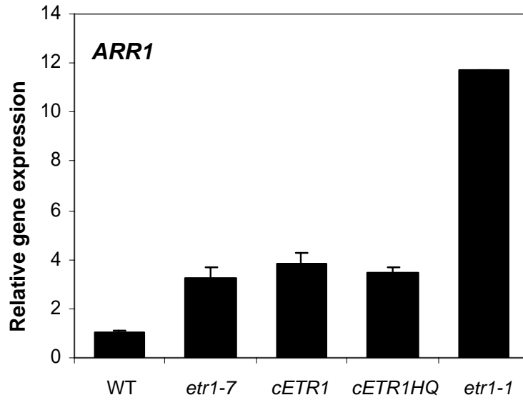
Figure S2. Relative expressions of ARR 1 (At3g16857) in the 4-days-old etiolated seedlings.
