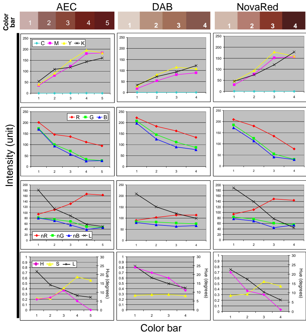
Supplementary Figure 1 Chromogen spectral characteristics. Color bars representing IHC stains without hematoxylin counterstain are defined by the individual channels of the different color models, CMYK, RGB, nRGB and HSL in each row.
