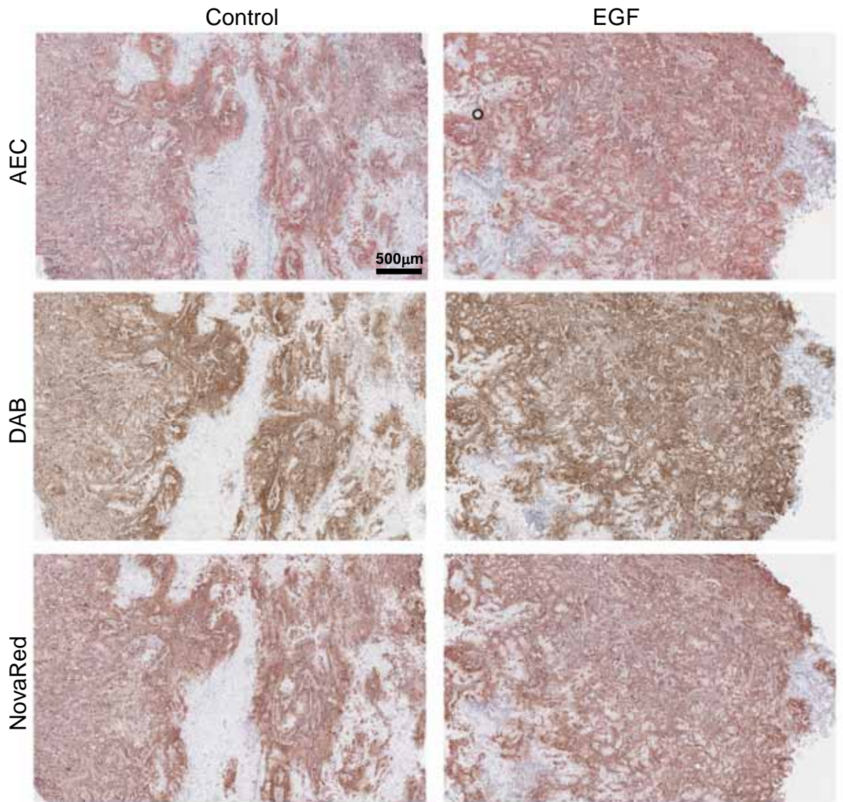
Supplementary Figure 2. Levels of S^{727} p-STAT3 was examined in a tumor xenograft specimen divided for EGF stimulation compared to control. Serial sections were stained with the different chromogens and hematoxylin counterstained.
