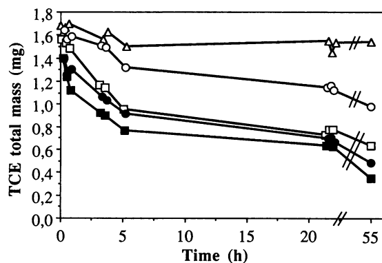
FIG. 2. TCE degradation in samples from the LMA and the LHS reactors measured with and without 20 mM formate. The datum points at 55 h represent final values beyond which no additional degradation occurred and were used to estimate TCE transformation capacity. \Delta , control; \circ and \bullet , LHS without and with formate, respectively; \square and \blacksquare , LMA without and with formate, respectively.
