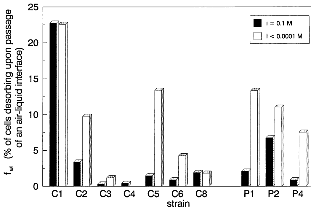
FIG. 3. Fraction of cells desorbing from Teflon beads in columns when an air-liquid interface was passed ( f_{ai} ). The two aqueous media tested were 0.1 M PBS and deionized water ( I , <0.0001 M).
