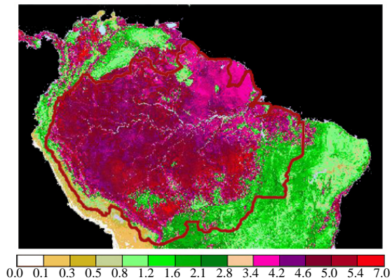
Annual Average Leaf Area Index
