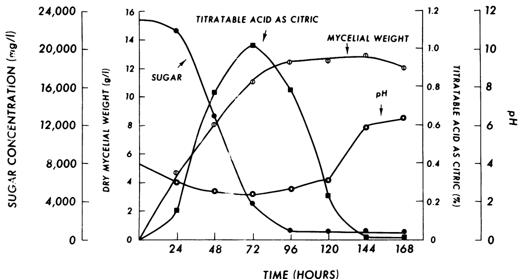
FIG. 1. Growth of A. niger on brewery spent grain liquor.
