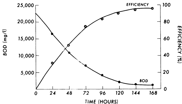
FIG. 2. BOD reduction in brewery spent grain liquor by A. niger .
