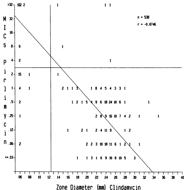
FIG. 2. Scattergram for pirlimycin MICs and clindamycin zone diameters (2 µg per disk) obtained in tests with gram-negative and -positive mastitis pathogens (the same strains used in Fig. 1). The horizontal line represents the MIC breakpoint ( \leq 2 µg/ml is susceptible), and the vertical line represents the disk diffusion breakpoint ( \geq 13 mm is susceptible).
