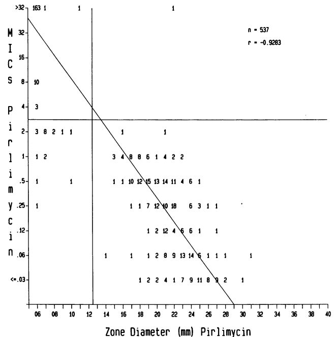
FIG. 1. Scattergram for pirlimycin MICs and zone diameters (2 µg/ml) obtained in tests with gram-negative and -positive mastitis pathogens and some human strains of staphylococci (n = 537). The horizontal line represents the MIC breakpoint (≤2 µg/ml is susceptible), and the vertical line represents the disk diffusion breakpoint (≥13 mm is susceptible). See the text for species tested. For the regression calculations, the extreme values (≥32 and ≤0.03 µg/ml and 6 mm) were excluded.
