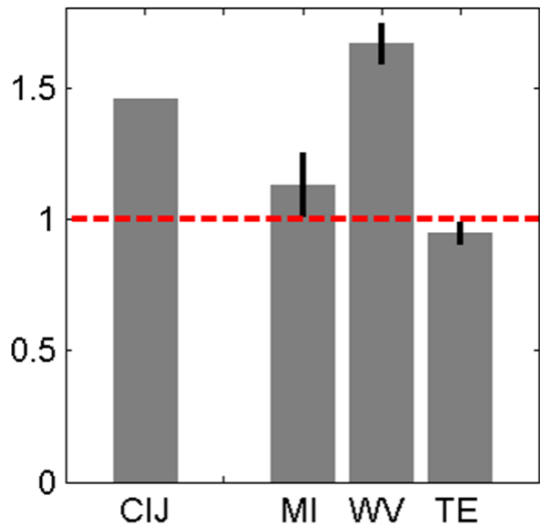
small-world index
