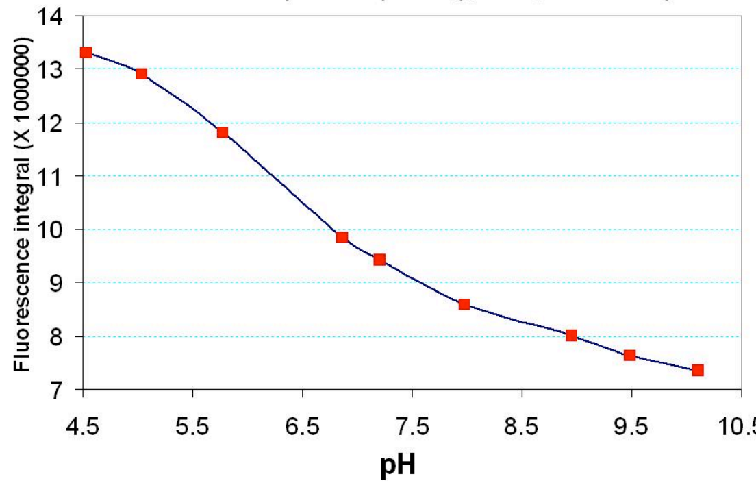
Fluorescence Response of (\text{DPA-C}_2)_2\text{-TPPS}_3 at different pH
