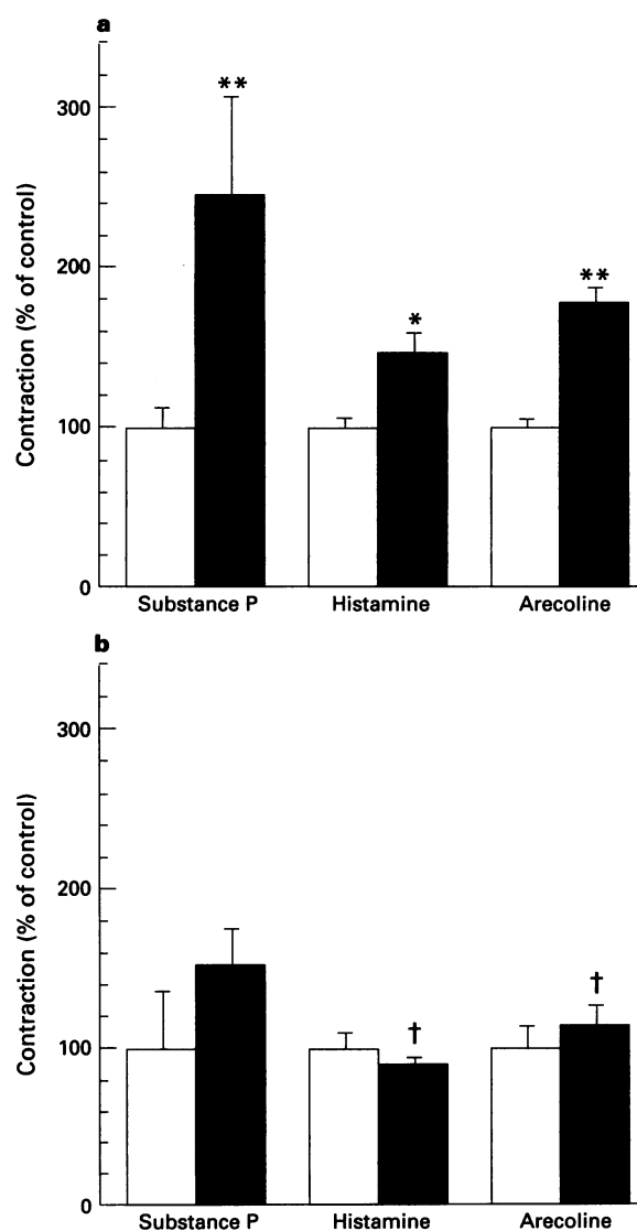
Figure 2 Maximal tracheal contractions (as % of control) in response to substance P, histamine and arecoline 4 days after inoculation with control solution (open columns) or PI-3 virus (solid columns) of animals (a) pretreated with vehicle (b) pretreated with capsaicin. * P < 0.05 ; ** P < 0.01 (Bonferroni) compared to the control inoculated group. † P < 0.05 (Bonferroni) compared with the virus inoculated groups in Figure 2a. The data are presented as mean \pm s.e. mean ( n = 8 ).
