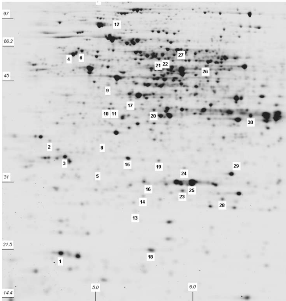
Figure S3 Overview of protein spots chosen for sequencing
