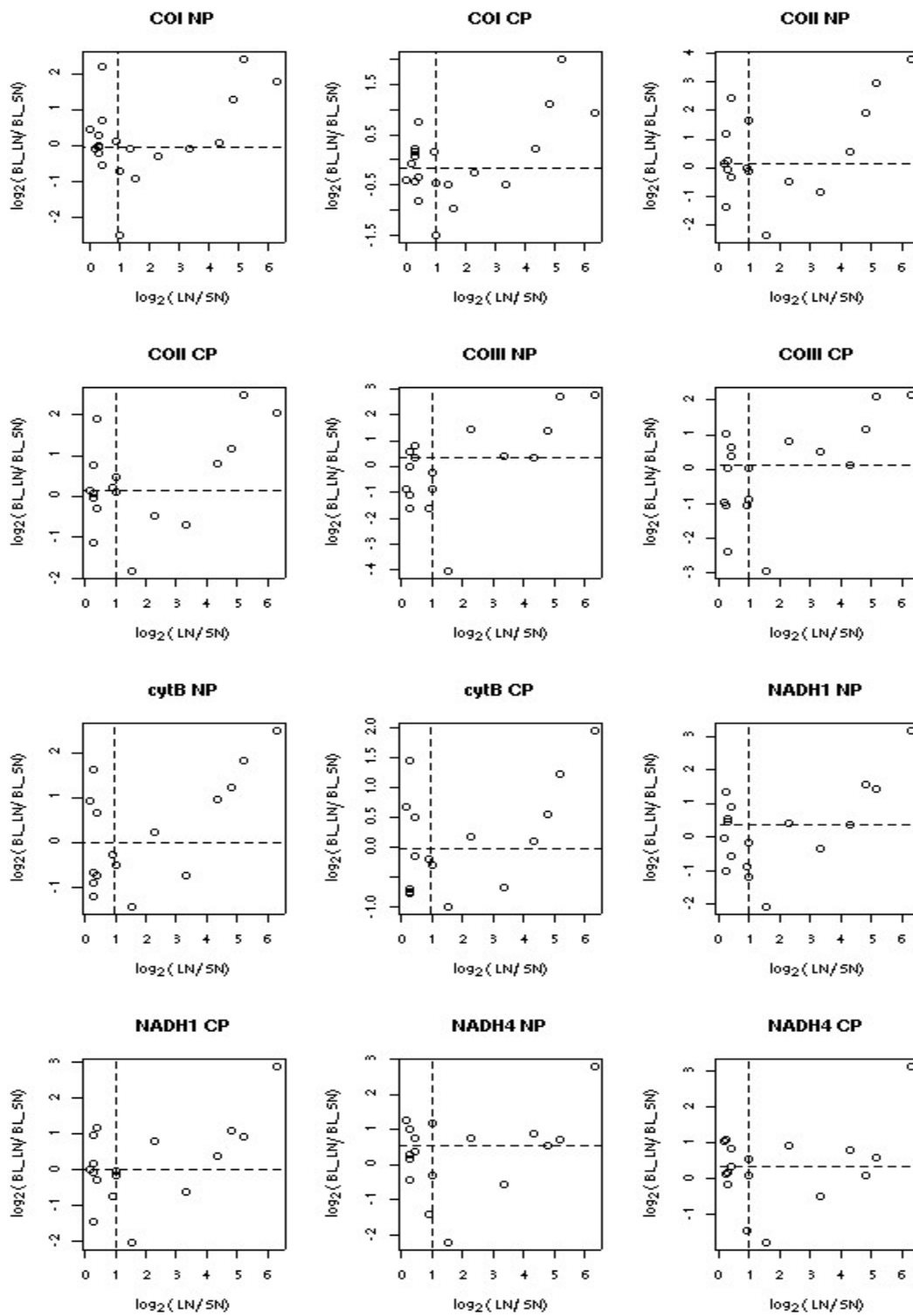
(b) Mitochondrial genes
