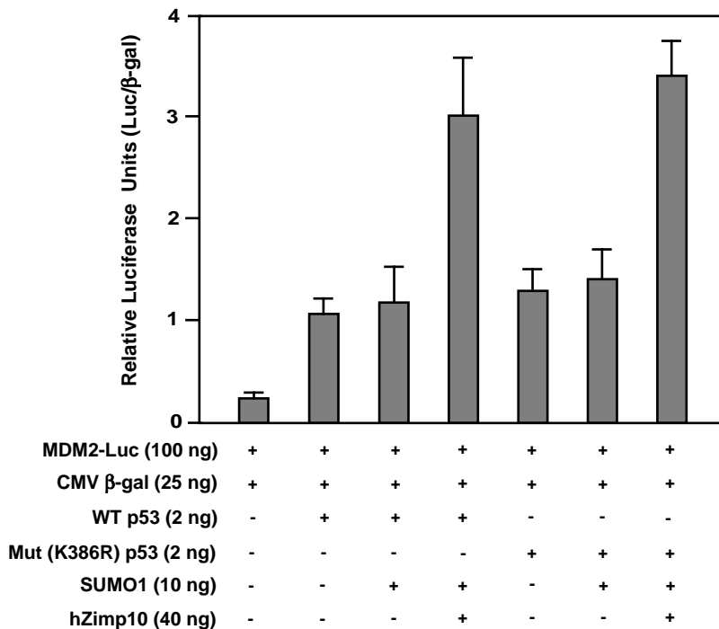
S-Figure 2. hZimp10 augments wild type and mutated p53 mediated transcription. Luciferase assays were performed on lysates from HEK293 cells transfected with different plasmids as indicated in the figure. The total amount of plasmid per well was normalized in all transfections by addition of pcDNA3 empty vectors. Luciferase activity is reported as relative light units and represented as mean \pm SD.
