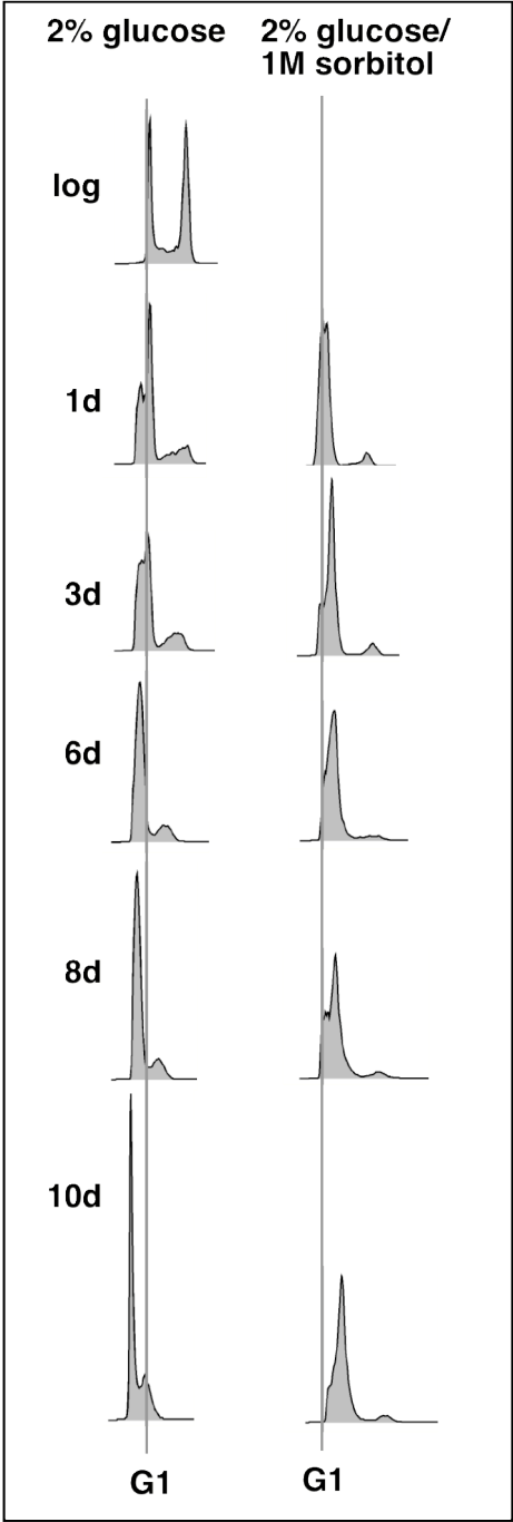
Weinberger Fig. S2. Effect of osmotic stress (1M sorbitol) on DNA content during medium depletion.
