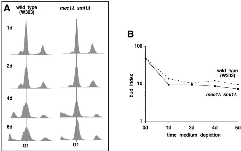
Figure S3 Weinberger et al. In the absence of the ribonucleotide reductase inhibitor Sml1, deletion of MEC1 does not alter the efficiency of G1 arrest during nutrient depletion. A. FACS measurements of DNA content in wild type and mec1Δ sml1Δ cells at various times of nutrient depletion (indicated at left of FACS profiles). B. Budding indices of these cells.
