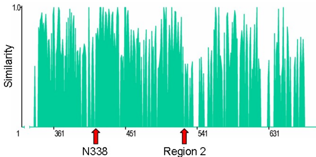
Supplemental Figure 2 online. Plot of amino acid similarity across the C-terminal domain of an alignment of 46 monoterpene synthases. Both N338 and region 2 fall into local similarity minima. Other minima coincide with either exposed loop regions or gaps in the amino acid alignment. Alignment and analysis of similarity were performed using the AlignX program of Vector NTI suite (Informax, Inc.).
