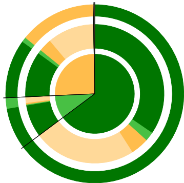
124 Prokaryotic Genomes
