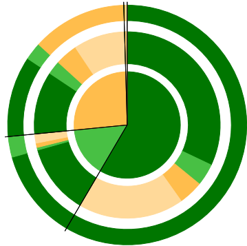
Archaeoglobus fulgidus
